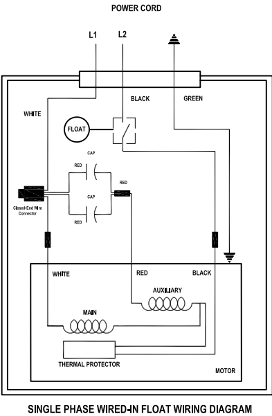
WIRING DIAGRAM FOR MODELS "WU2702"
