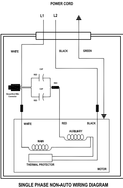
WIRING DIAGRAM FOR MODELS "V2702"
